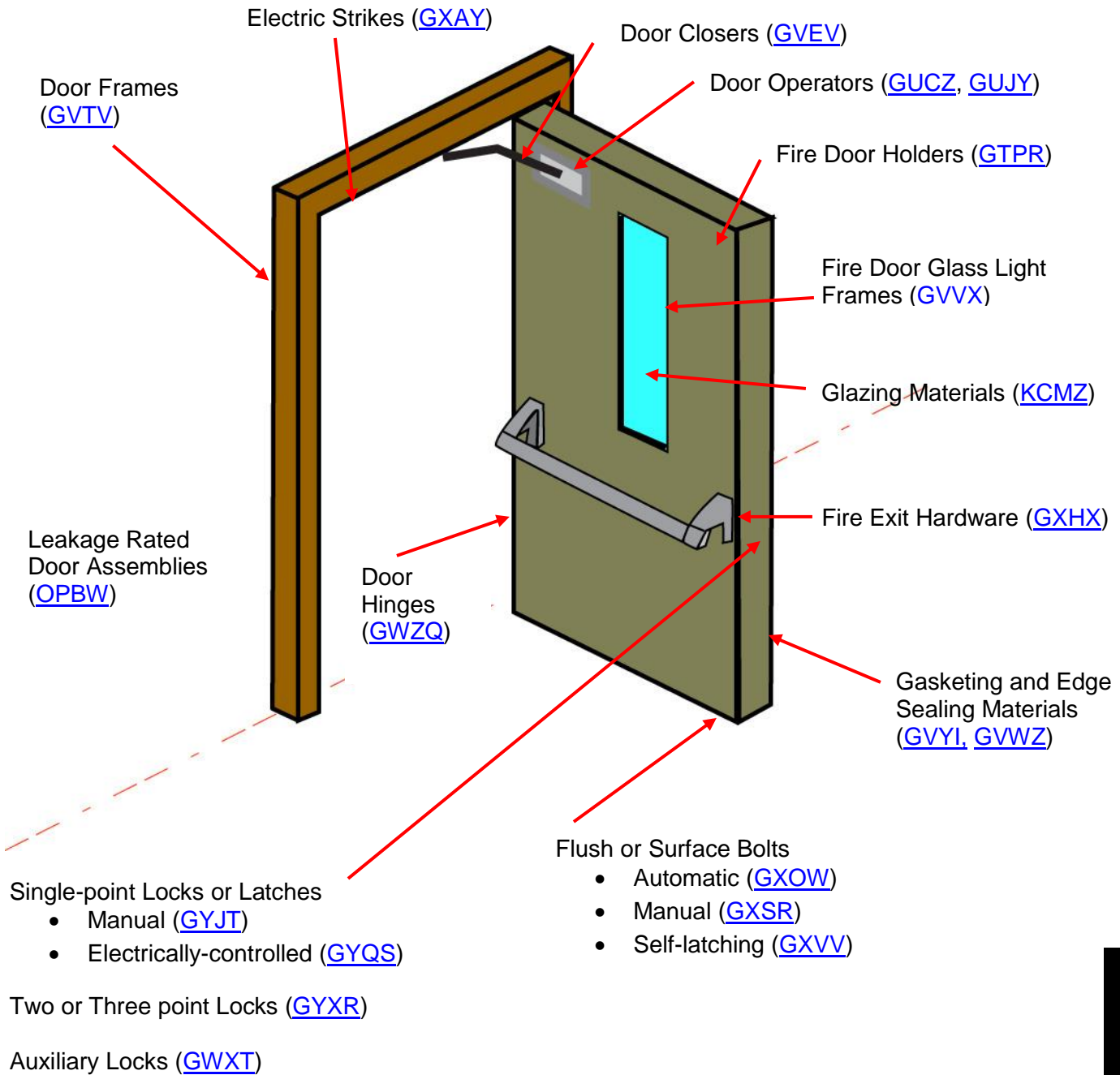
Swinging-type Fire Door ( GSZN for UL 10C, GSYX for UL 10B)
